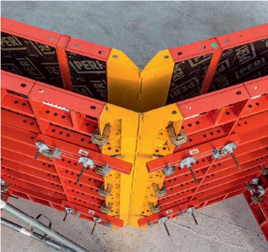
With the LIWA Articulated Corner, obtuse corners from 75° to 165° are formed; thereby compensation walers are to be mounted on the external corners.
